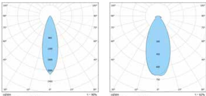
S3 (NEMA 3)
